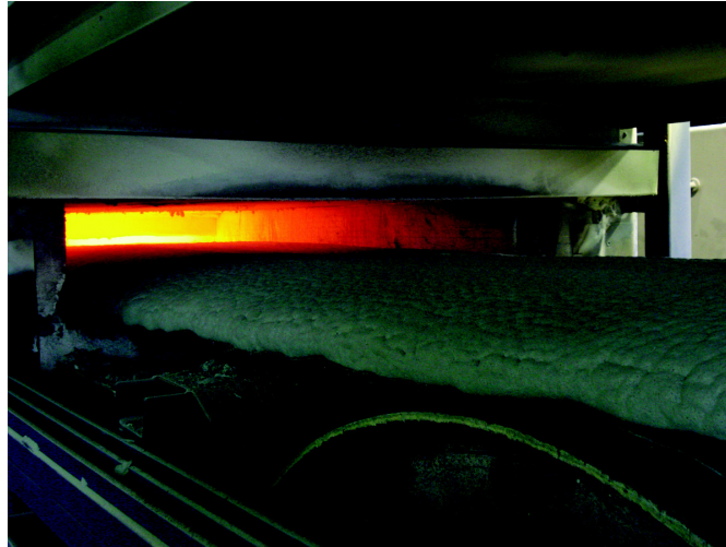
Figure 1 Exit point of the glass foam “cake” from the furnace. The expanded compound cools down from about 900°C to ambient temperatures. (Reproduced by permission of Misapor AG.)
